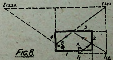
Diagram showing the path of a ray reflected in one plane by four mirrors arranged like the cushions of a billiard table.
