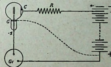
Fig. 4. Circuit for measuring Sensitivity of a Photo-Electric Cell.
