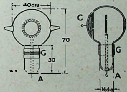
Fig. 2. Dimensions (in millimetres) of the Lindemann Cell.
