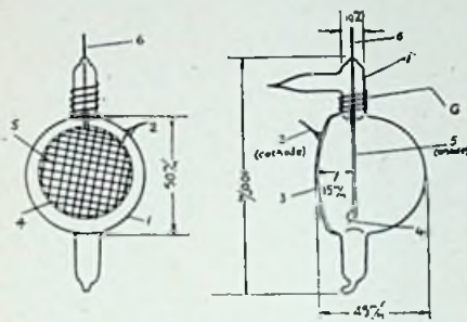
Fig. 7. Illustrating the gauze type of Photo-Electric Cell.
