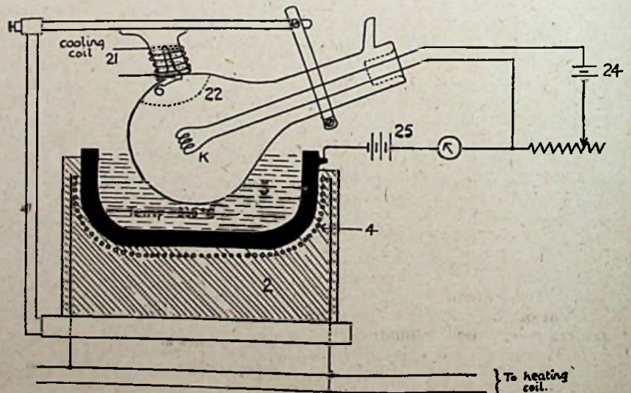
Fig. 6.—Process of manufacture of Zworykin Cell.
